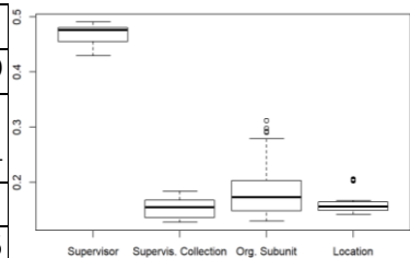
Figure 1: Cramer’s V correlations.
